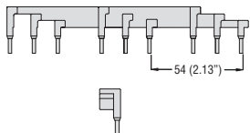
Connection busbars 54mm/2.13" spacing SMX90 42 - SMX90 43 - SMX90 44
