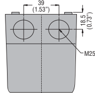
Drilling for surface fixing
