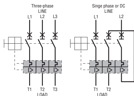
MOTOR PROTECTION CIRCUIT BREAKERS SM1A... - SM1B... - SM1C... and SM2A... - SM3A... and LMS25...
